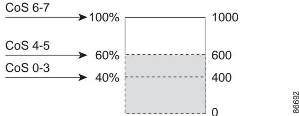
Figure 33-7 WTD and Queue Operation
