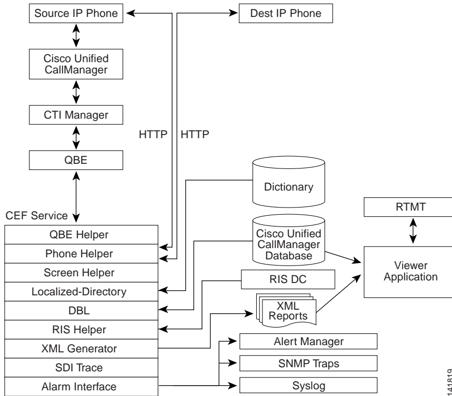
Figure 29-1 Using the Cisco Extended Functions Service Architecture
