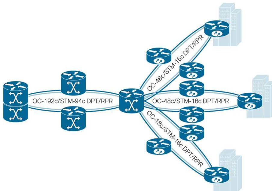
Figure 3. RPR Applications
