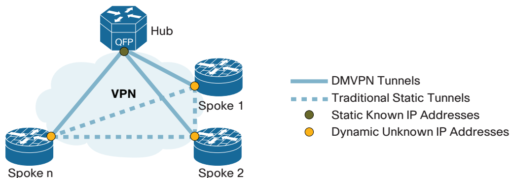
Figure 5. DMVPN
