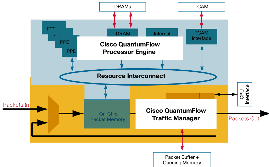
Figure 3. Cisco QuantumFlow Processor Major Block Diagram
