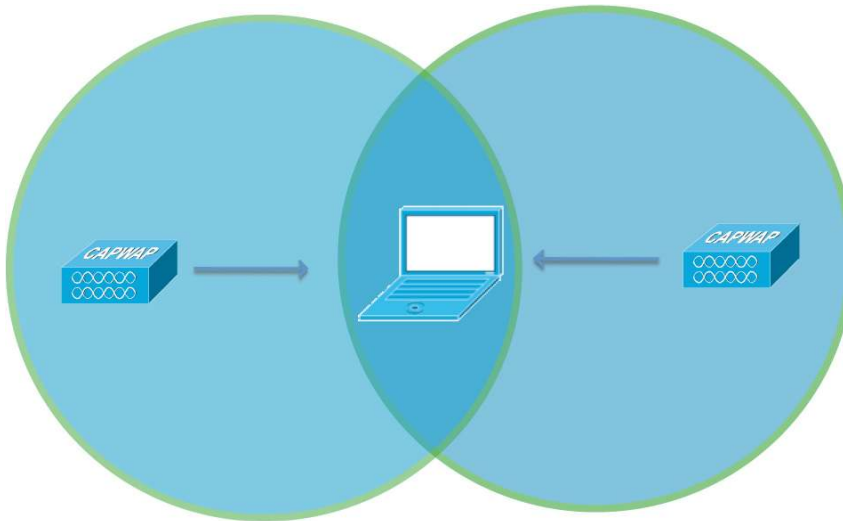
Figure 8. Co-Channel Interference
