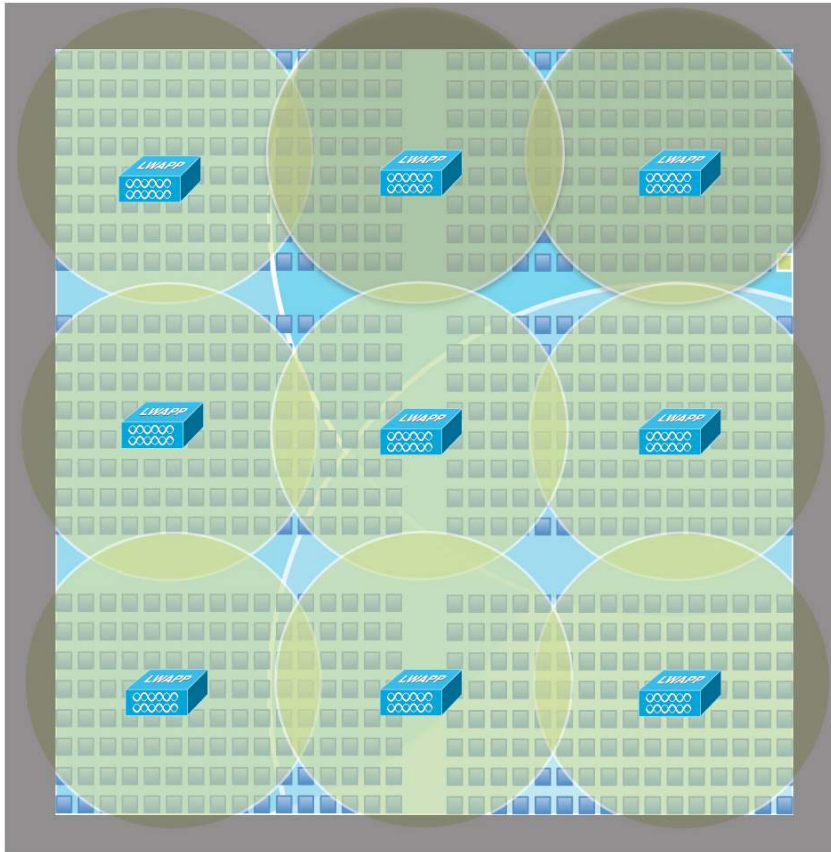
Figure 13. Nine AP WLAN Deployment
