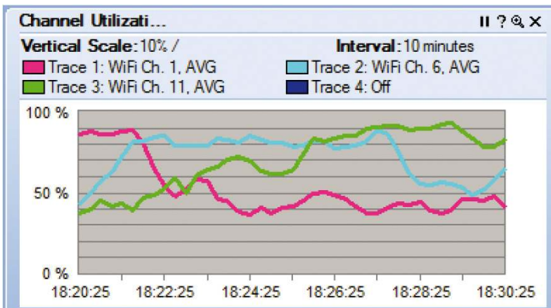
Figure 16. Duty Cycle Results in Room A
