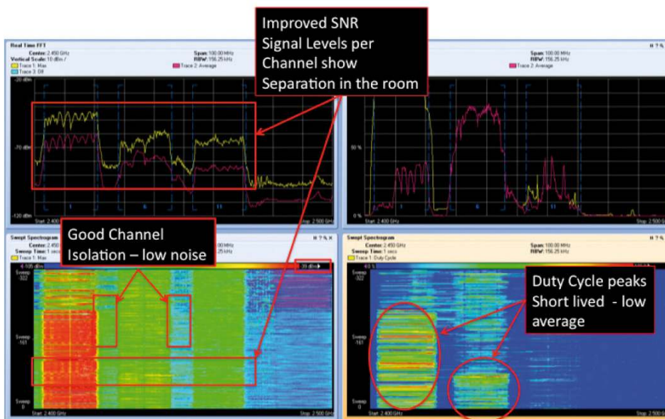
Figure 19. Spectrum View of Room B
