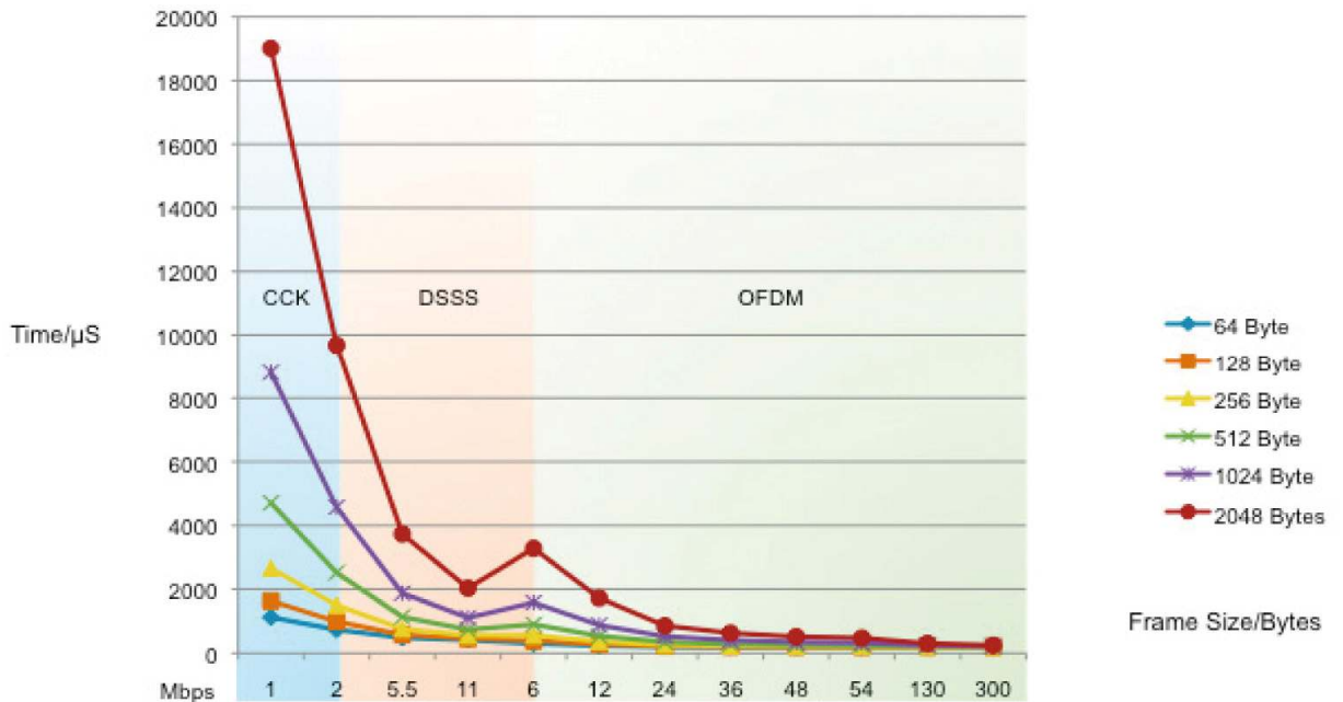
Figure 5. Per Frame Channel Utilization, Frame Sizes, and Data Rates in a WLAN
