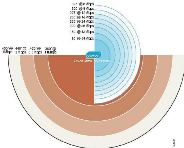
Figure 9. WLAN Coverage Model Based on Data Rates
