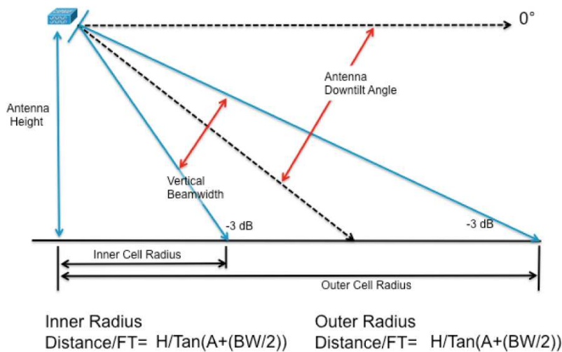
Figure 12. Adjusting Directional Antenna Using Downtilt
