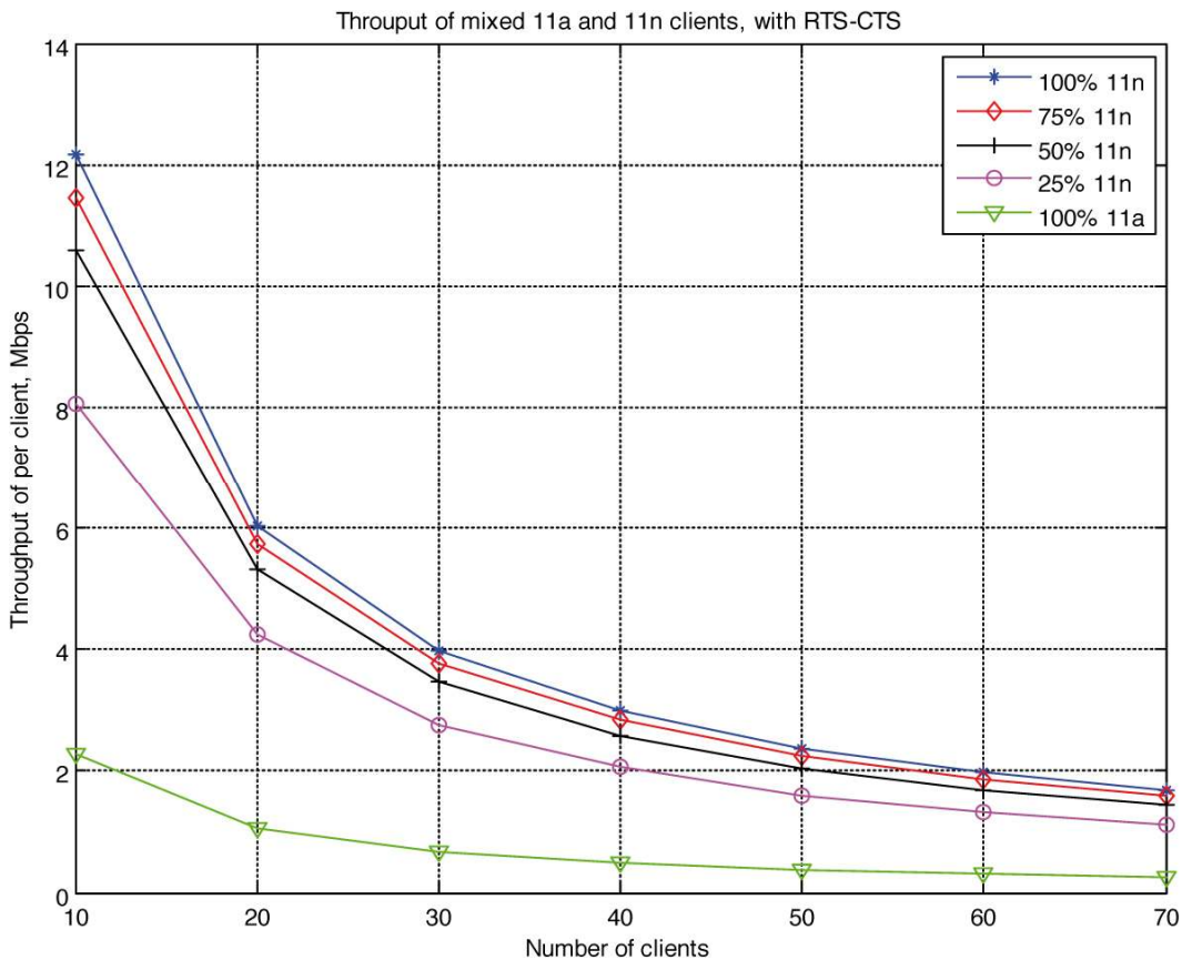
Figure 4. Mixed Wireless Client Protocol Performance in a Cell (802.11a/g/n Data Rates)
