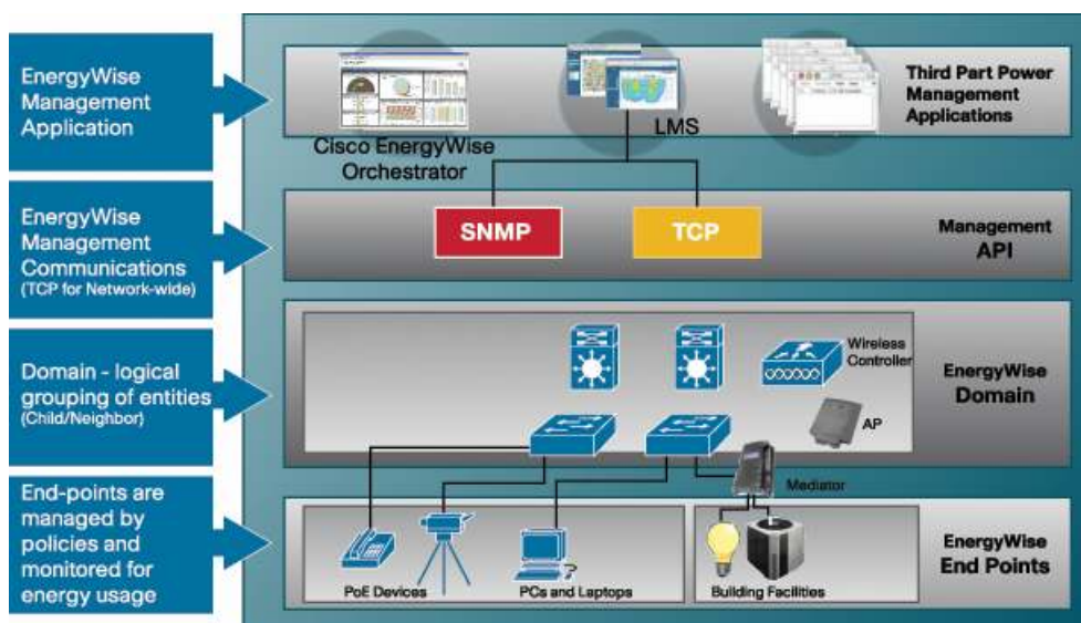
Figure 4. Cisco EnergyWise Intelligent Network Framework
